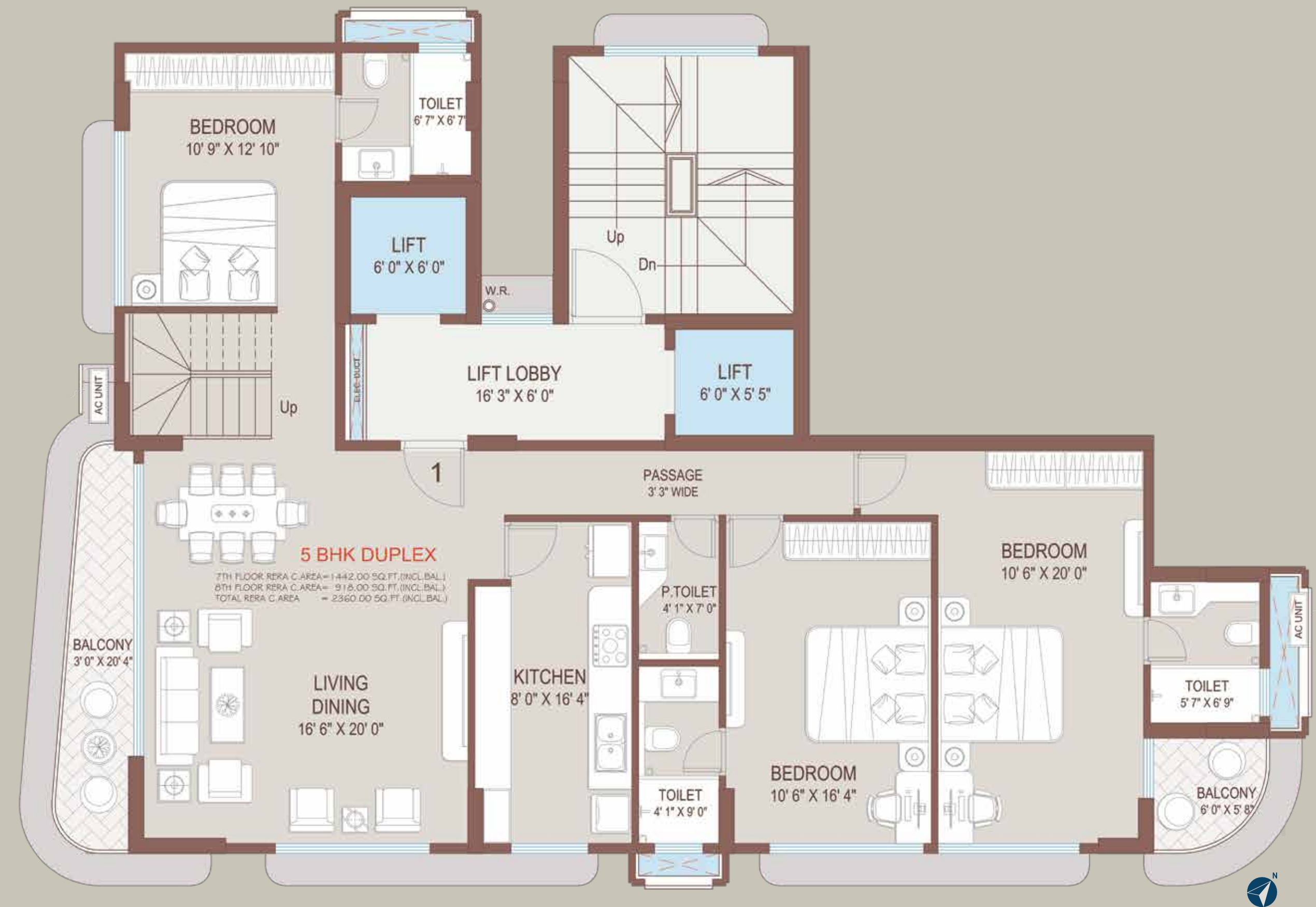
7 th Floor Plan
