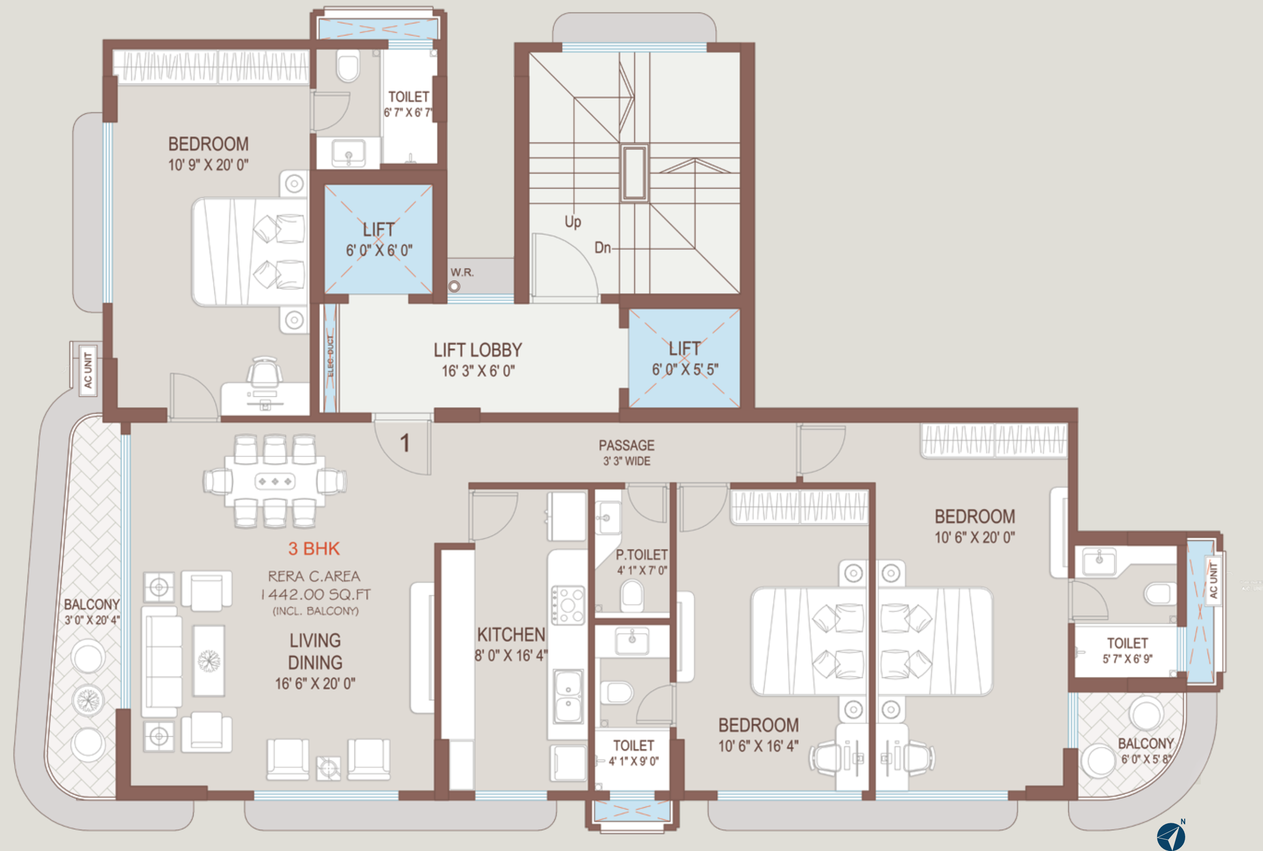
1 st to 6 th Floor & 9 th to 11 th Floor Plan
