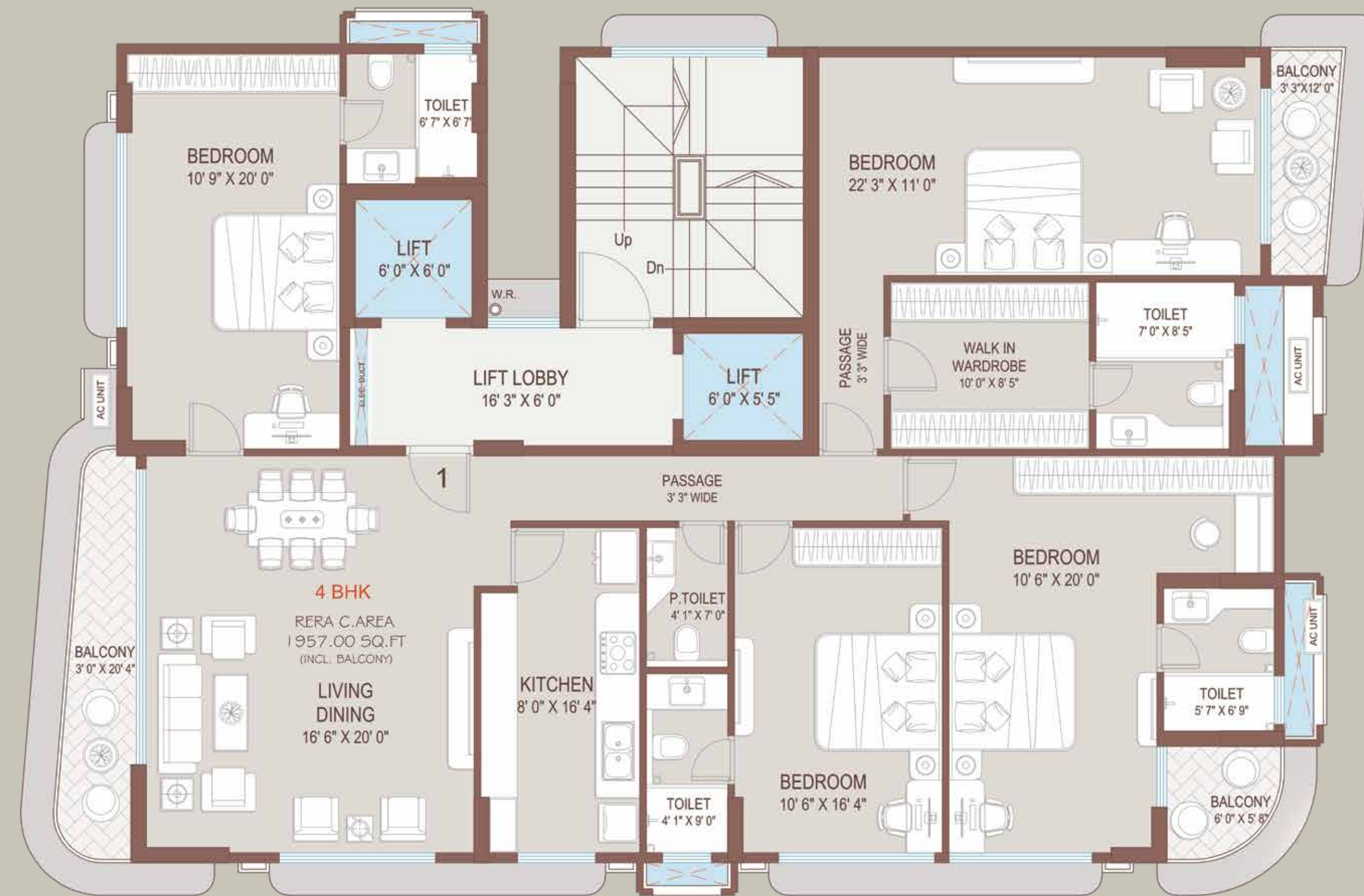
14 th to 15 th Floor Plan
